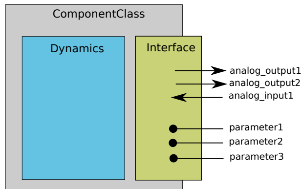
Figure 1: ComponentClass Overview
